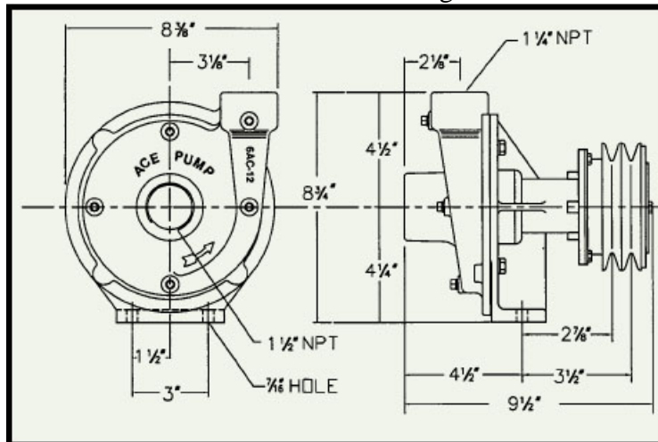
Dimension Drawing
