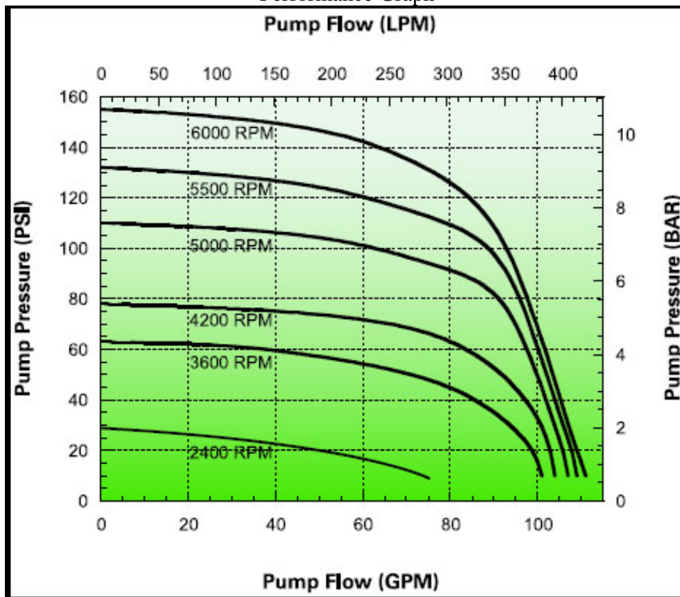
Performance Graph
